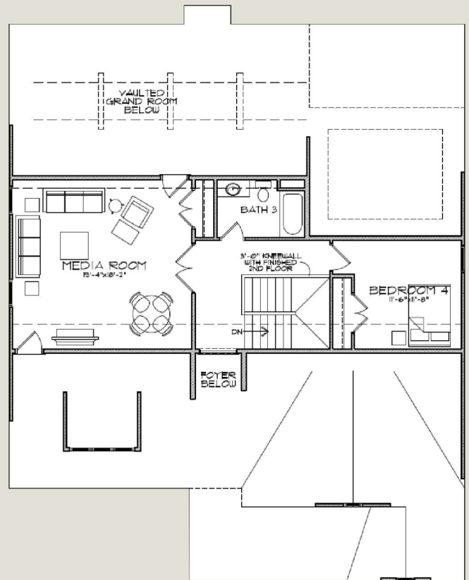
Second Level
