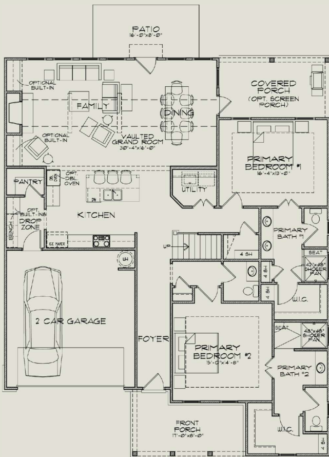
Main Level
