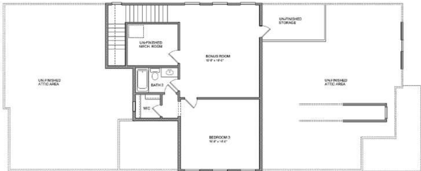
Second Floor
