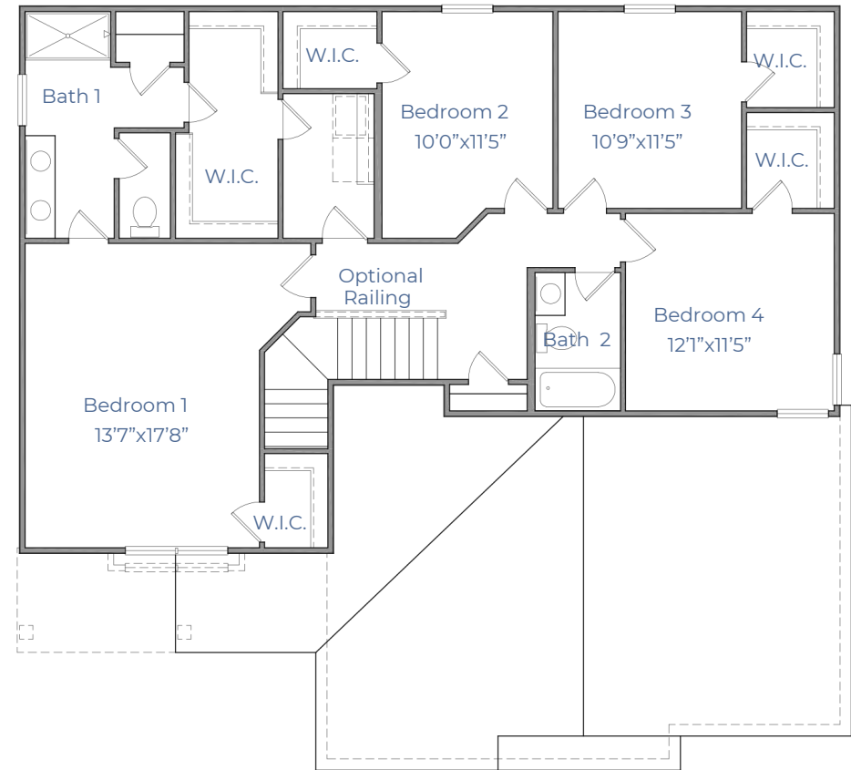
SECOND FLOOR
