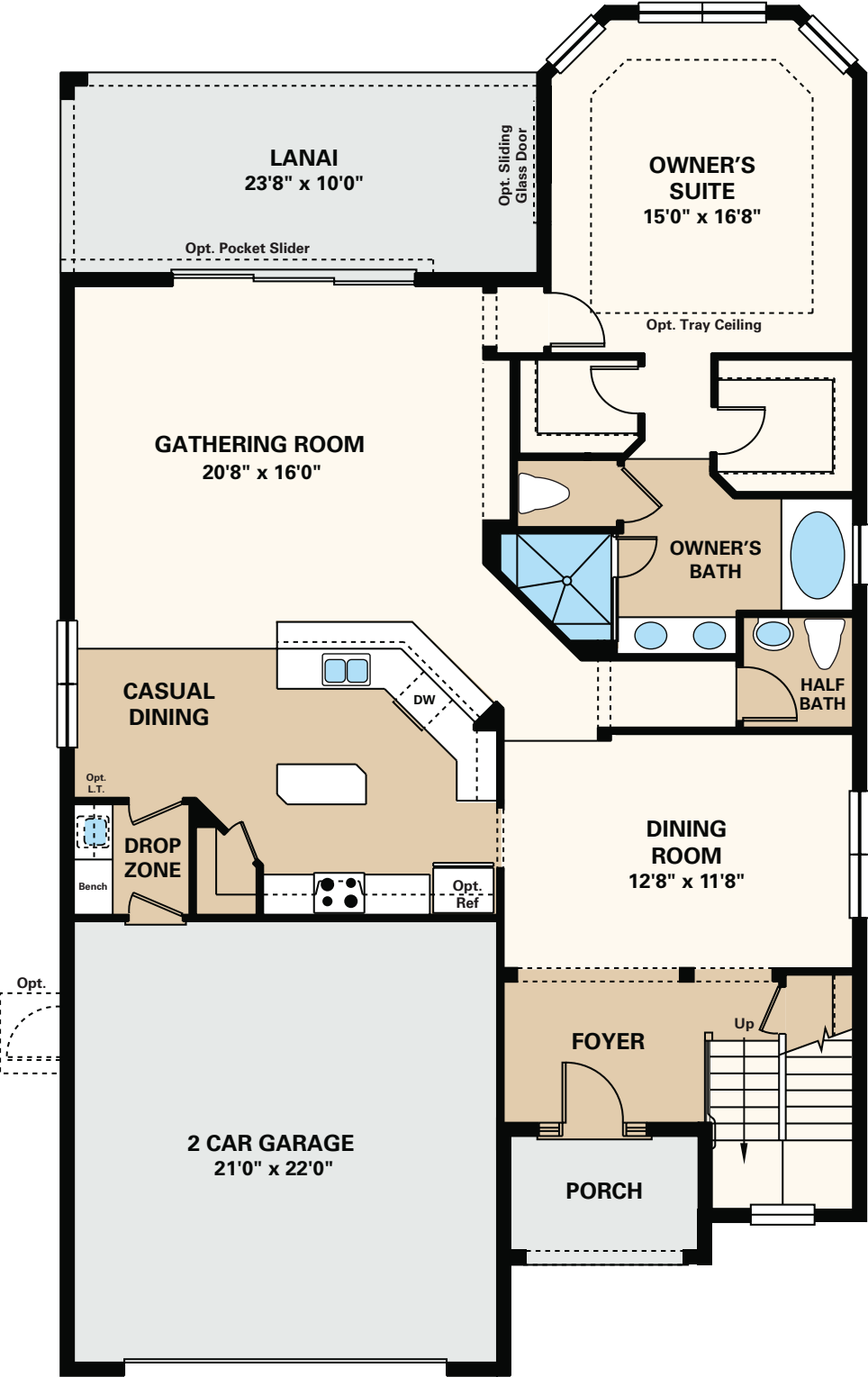
FIRST FLOOR
