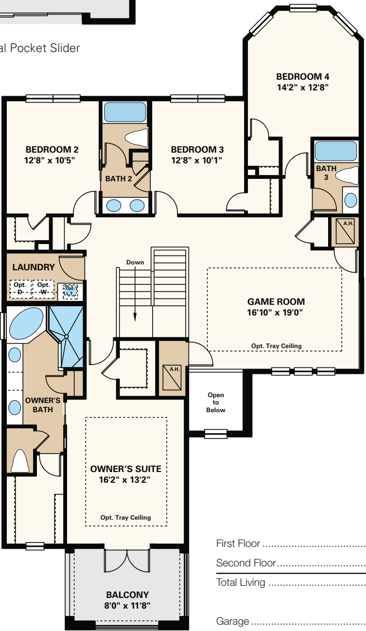
SECOND FLOOR
