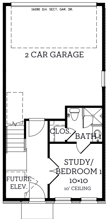
First Floor 339 sq.ft.
