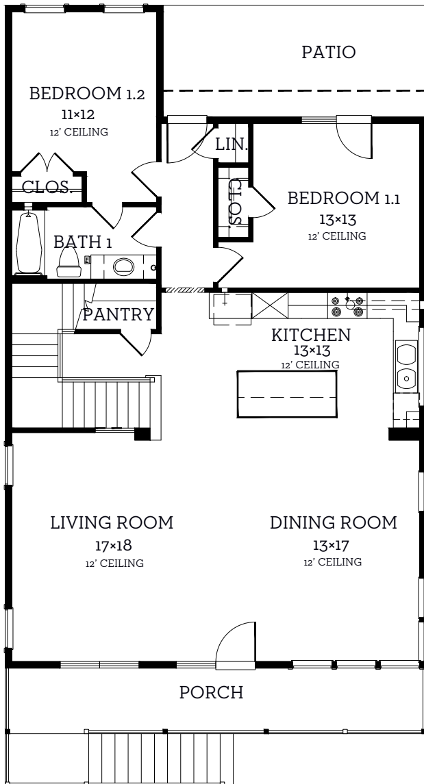
First Floor 1443 sq.ft.
