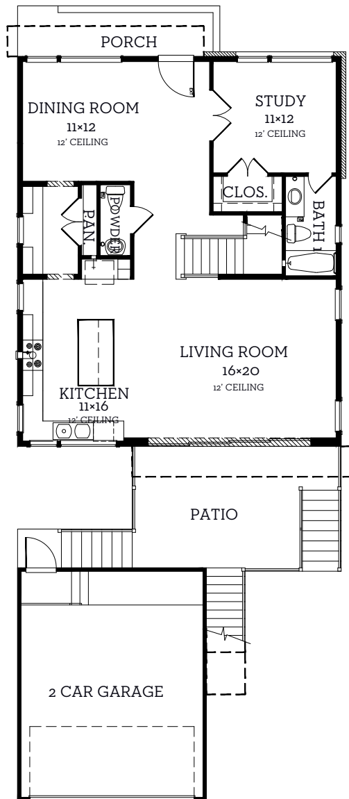
First Floor 1244 sq.ft.
