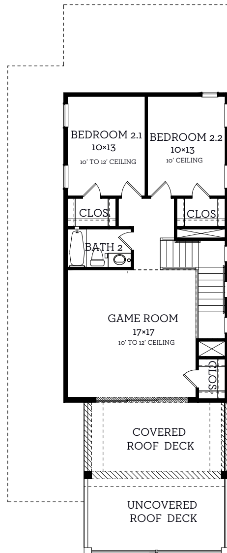
Second Floor 809 sq.ft.
