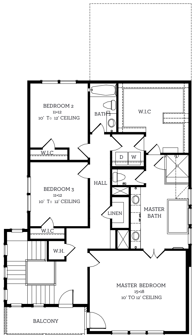
Second Floor 1347 sq.ft
