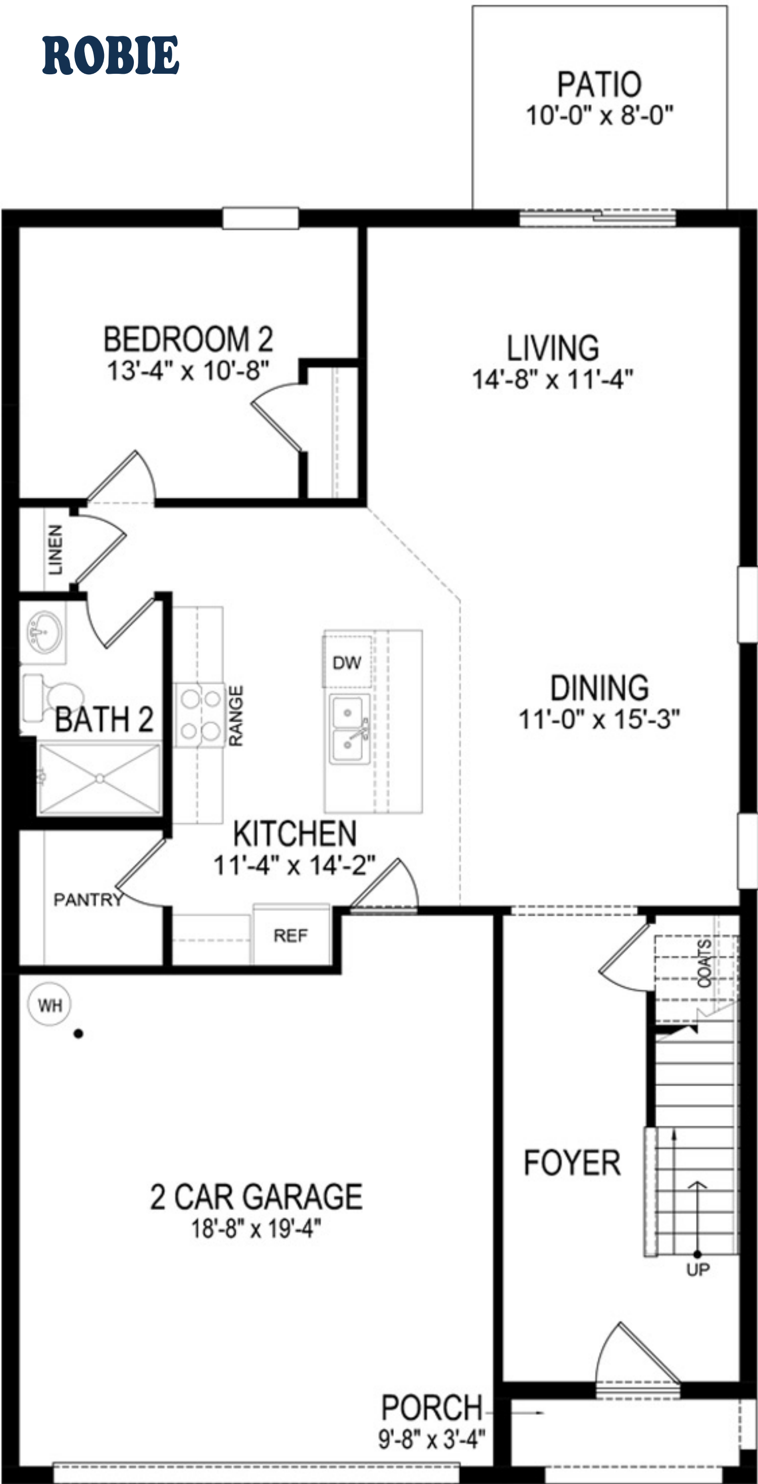
FIRST FLOOR
