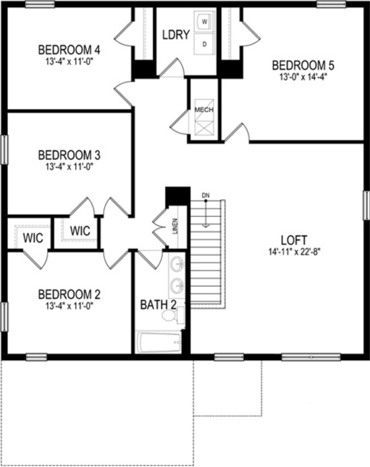
SECOND FLOOR
