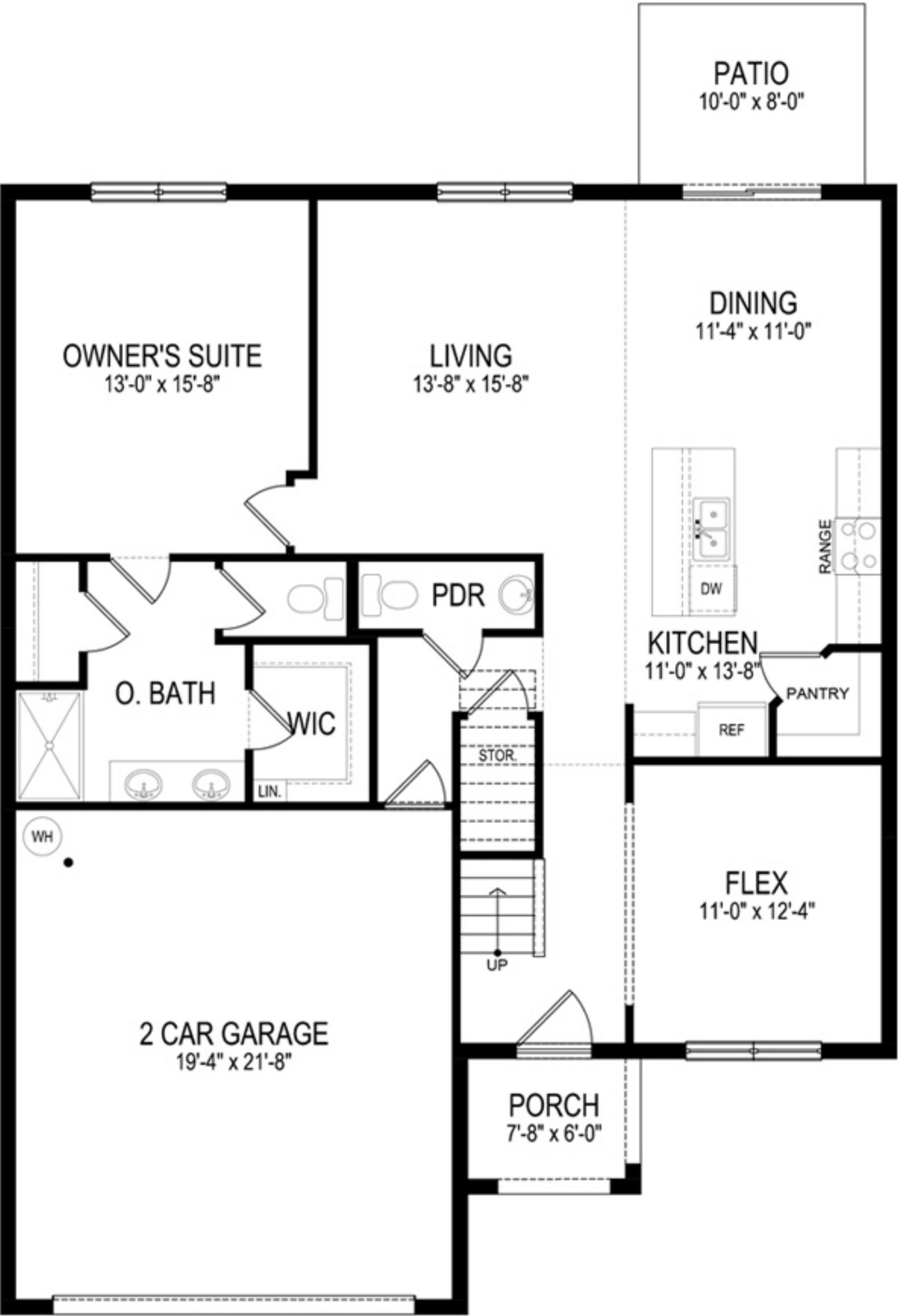
FIRST FLOOR
