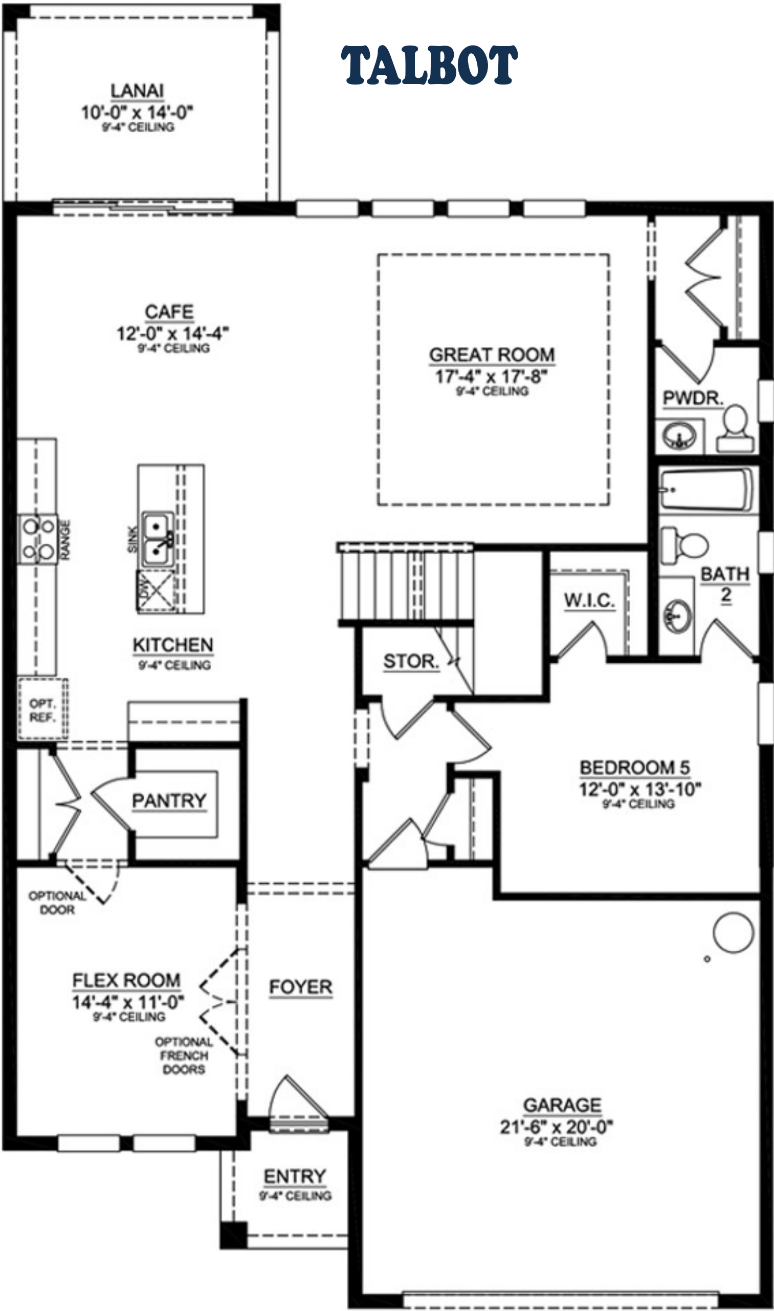
1ST FLOOR PLAN - ELEVATION G
