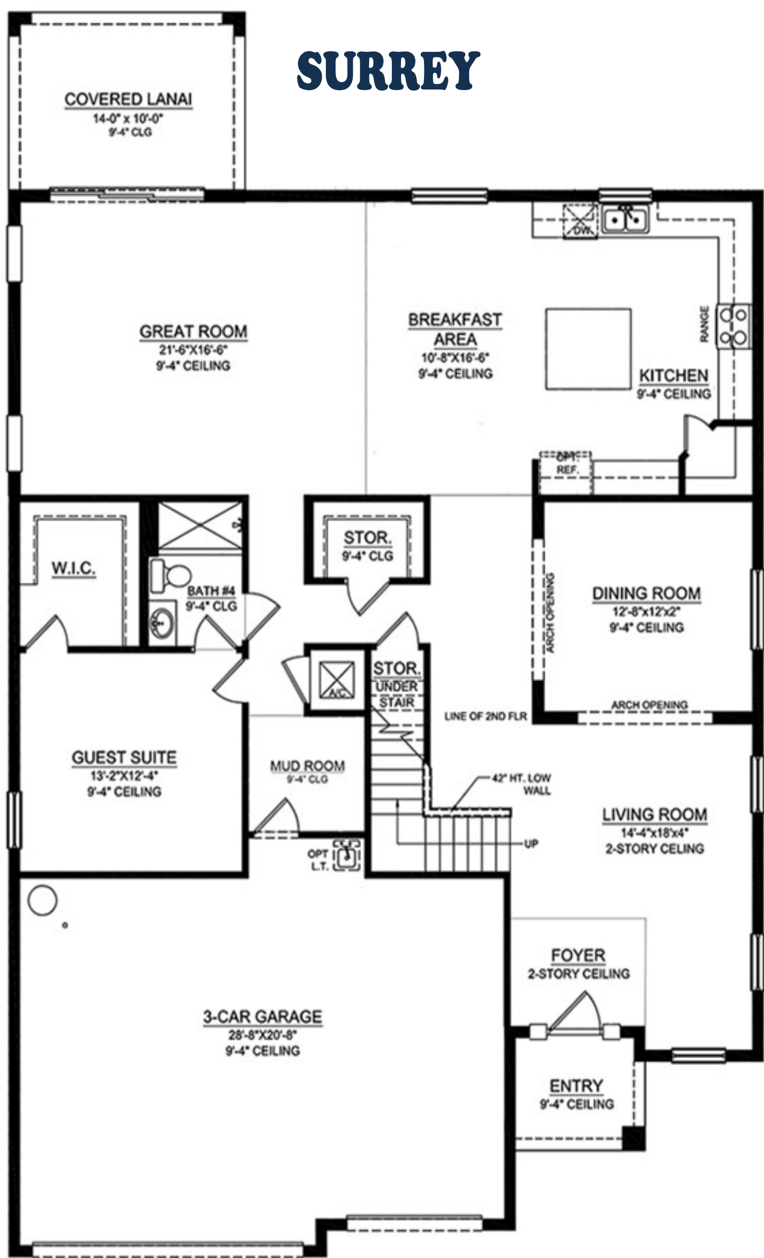
First Floor - Elevation G
