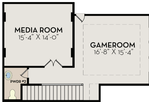
OPT. SECOND FLOOR 603 SQ. FT.
